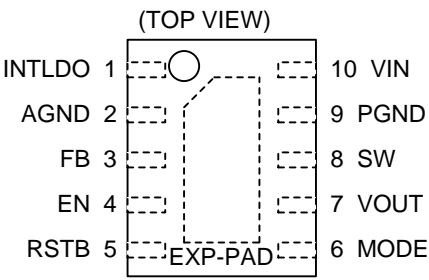
Figure 3. Pin Configuration
