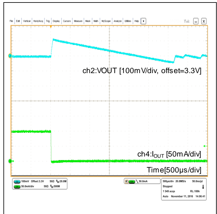
Figure 20. Transient Response ( V_{IN}=2.4V , MODE=H: Auto-PFM/PWM, Output current 1mA<->100mA)
