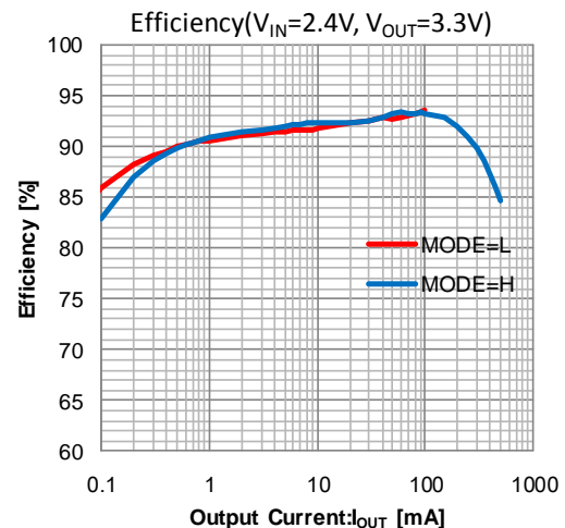
Figure 2. Efficiency
