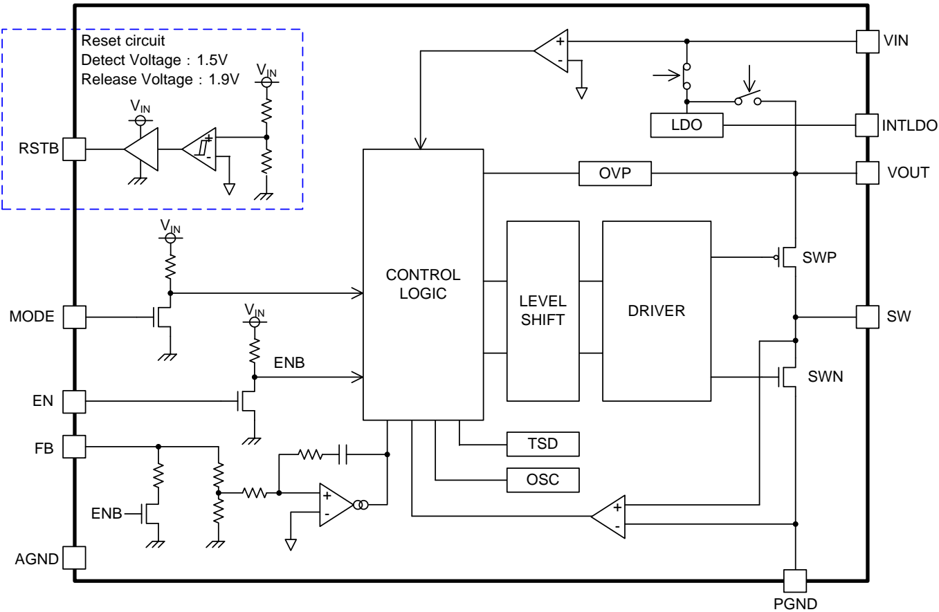
Figure 4. Circuit Block
