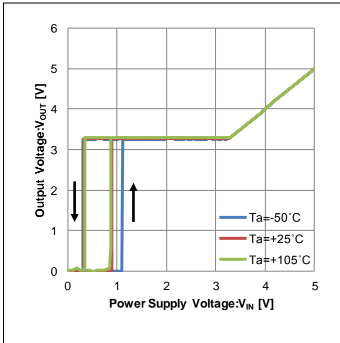
Figure 9. Output Voltage vs Power Supply Voltage ("Line Regulation", MODE=H: Auto-PFM/PWM, 3.3k \Omega resistive load)
