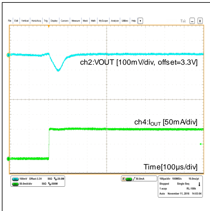
Figure 19. Transient Response ( V_{IN}=2.4V , MODE=H: Auto-PFM/PWM, Output current 1mA<->100mA)
