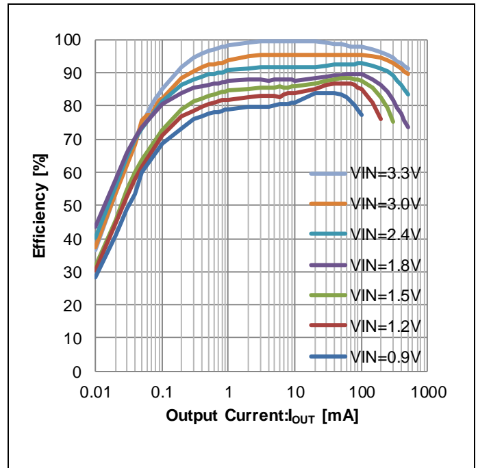
Figure 6. Efficiency vs Output Current (MODE=H: Auto-PFM/PWM)
