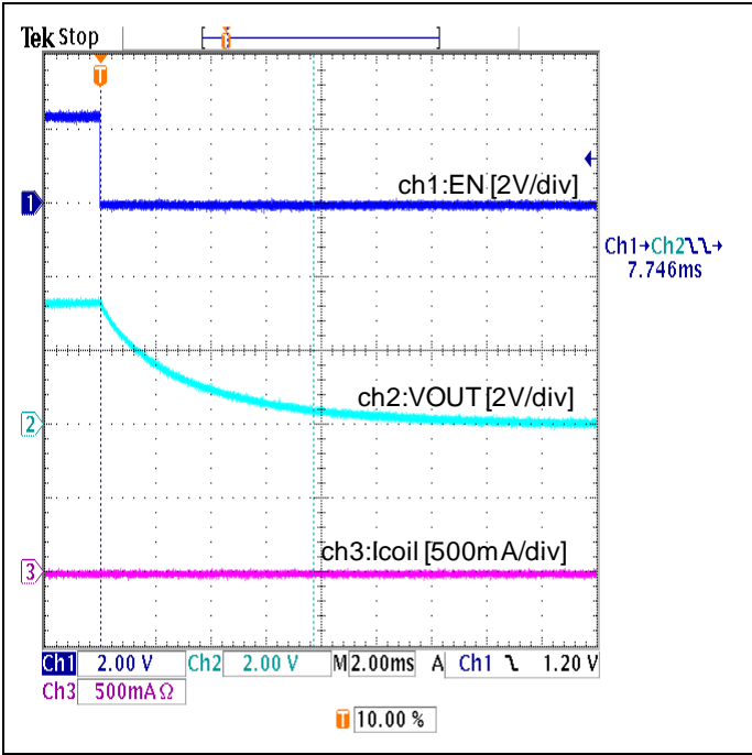
Figure 26. Shutdown Waveform ( V_{IN} =2.4V, Output current=0mA, MODE=H: Auto-PFM/PWM)
