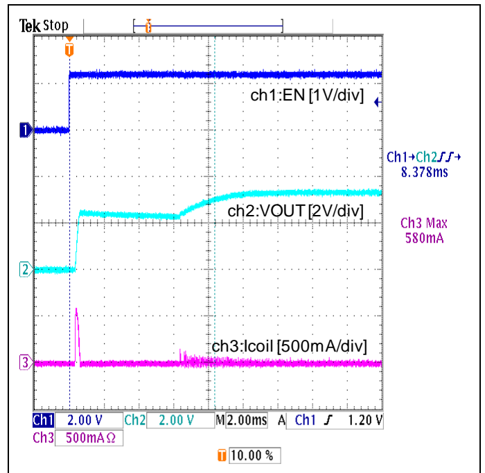
Figure 24. Start-up Waveform ( V_{IN}=2.4V , 3.3k\Omega resistive load, MODE=H: Auto-PFM/PWM)
