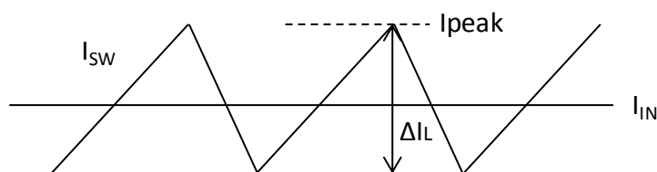
Figure 32. Switching Current
