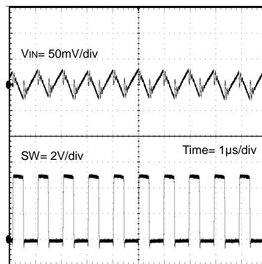
Figure 33. Input Ripple ( V_{IN}=5V , V_{OUT}=1.8V , I_{OUT}=3A )
