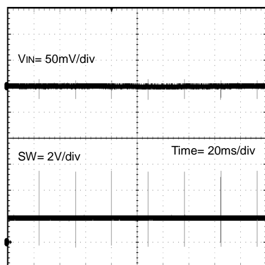
Figure 32. Input Ripple ( V_{IN}=5V , V_{OUT}=1.8V , I_{OUT}=0A )
