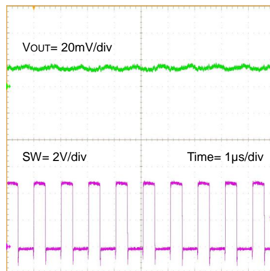
Figure 31. Output Ripple ( V_{IN}=5V , V_{OUT}=1.8V , I_{OUT}=3A )
