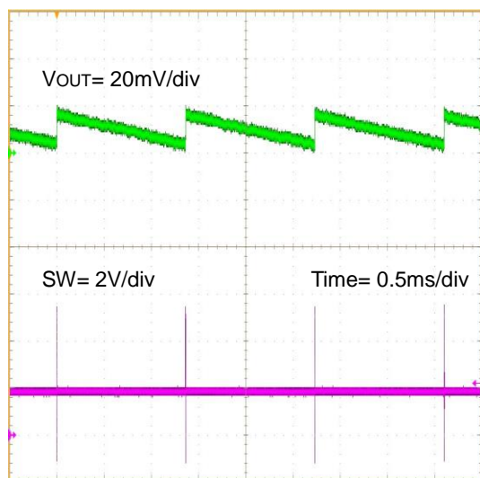
Figure 30. Output Ripple ( V_{IN}=5V , V_{OUT}=1.8V , I_{OUT}=0A )
